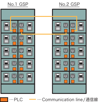
Distributed arrangement 分散型配置図
